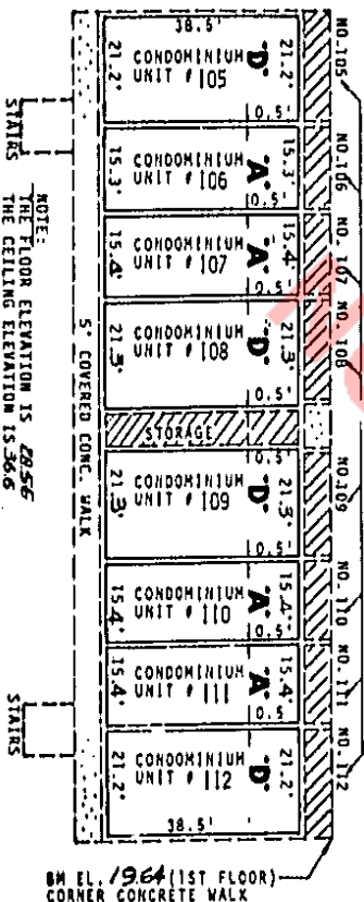
2ND FLOOR
